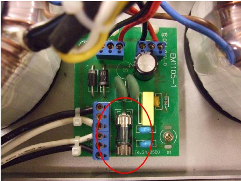
PSU PCB – value marked on PCB
