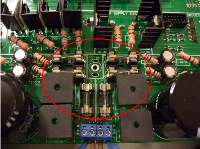
Main board – values are marked on PCB
